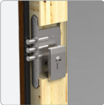
3-bolt class 6 additional GERDA ZW 500 lock
